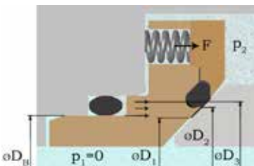
The seats with DOUBLE PISTON EFFECT are not self-relieving
