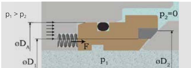
The seat is pushed against the ball permanently by the spring force (F) and by the piston effect - from the overpressure of the fluid in the valve bore acting on the annulus defined by \phi D_A and \phi D_1 .
