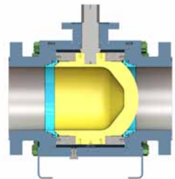
Fig. 8 Pig ball valve
